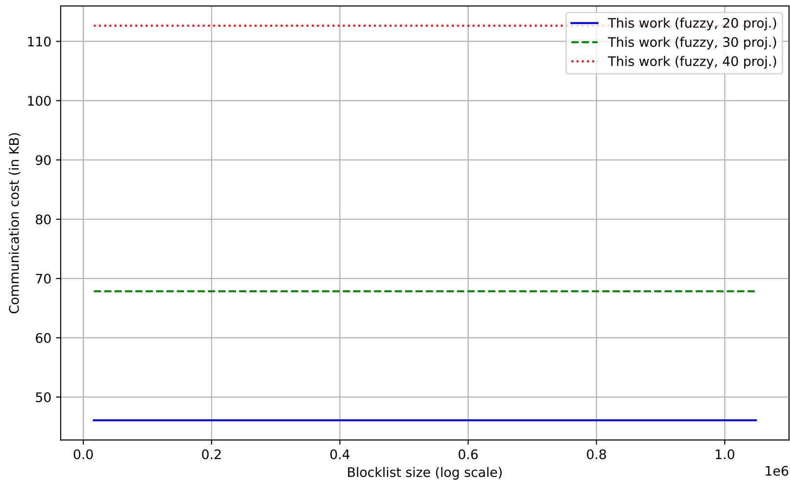
Communication cost vs. Blocklist size
